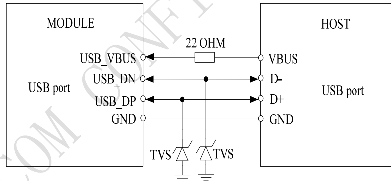
Figure 25: USB interface
