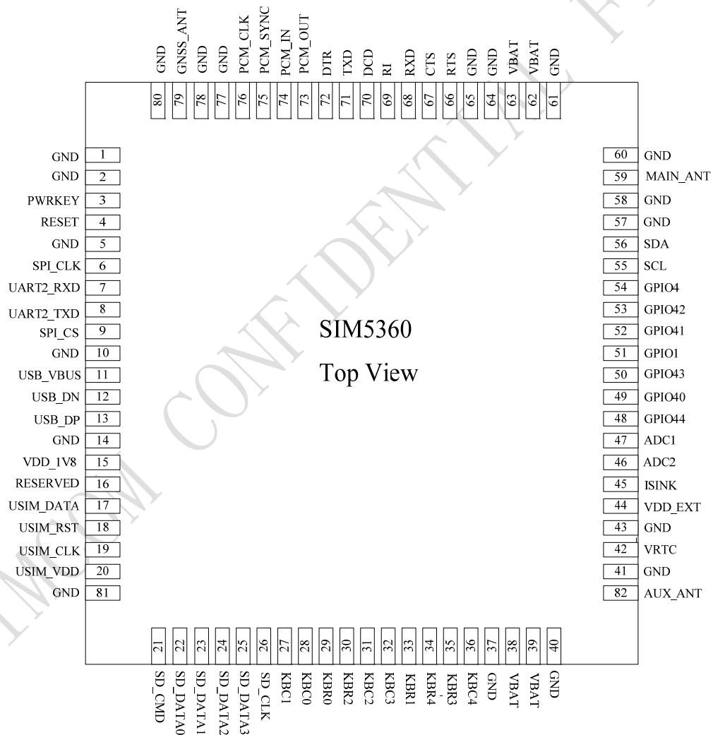
Figure 2: Pin view
