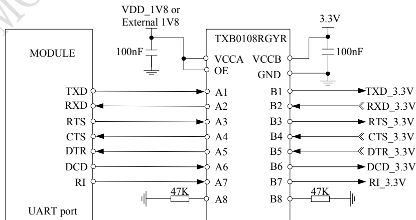
Figure 20: Reference circuit of level shift
