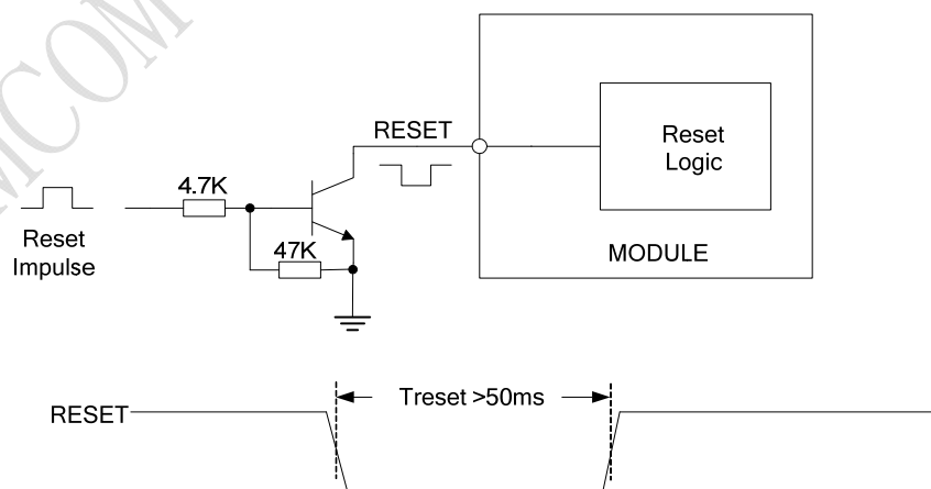
Figure 38: Reset circuit
