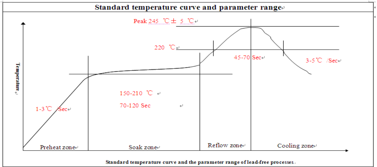
Figure 42: The ramp-soak-spike reflow profile of SIM5360
