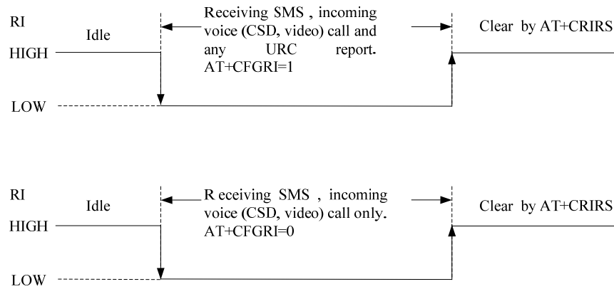
Figure 18: RI behaviour in NULL Modem
