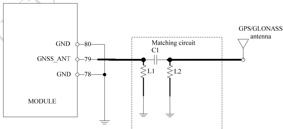
Figure 36: Passive antenna circuit (Default)
