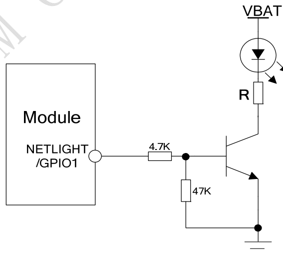
Figure 26: Application circuit
