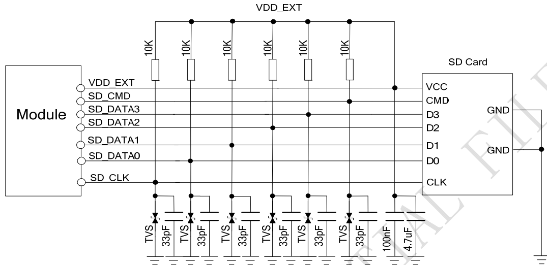
Figure 21: SD interface circuit
