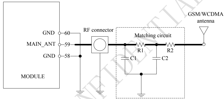
Figure 39: Antenna matching circuit (MAIN_ANT)
