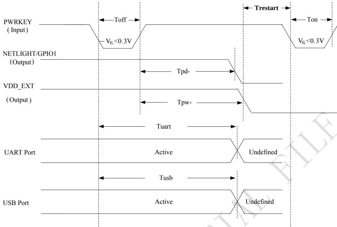
Figure 15: Power off timing sequence
