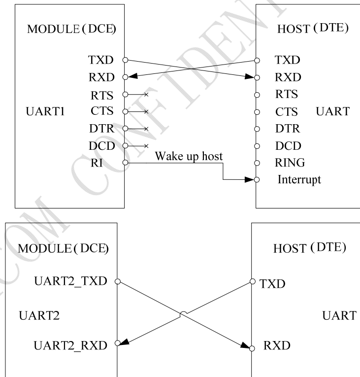
Figure 17: Null modem (UART1 and UART2)
