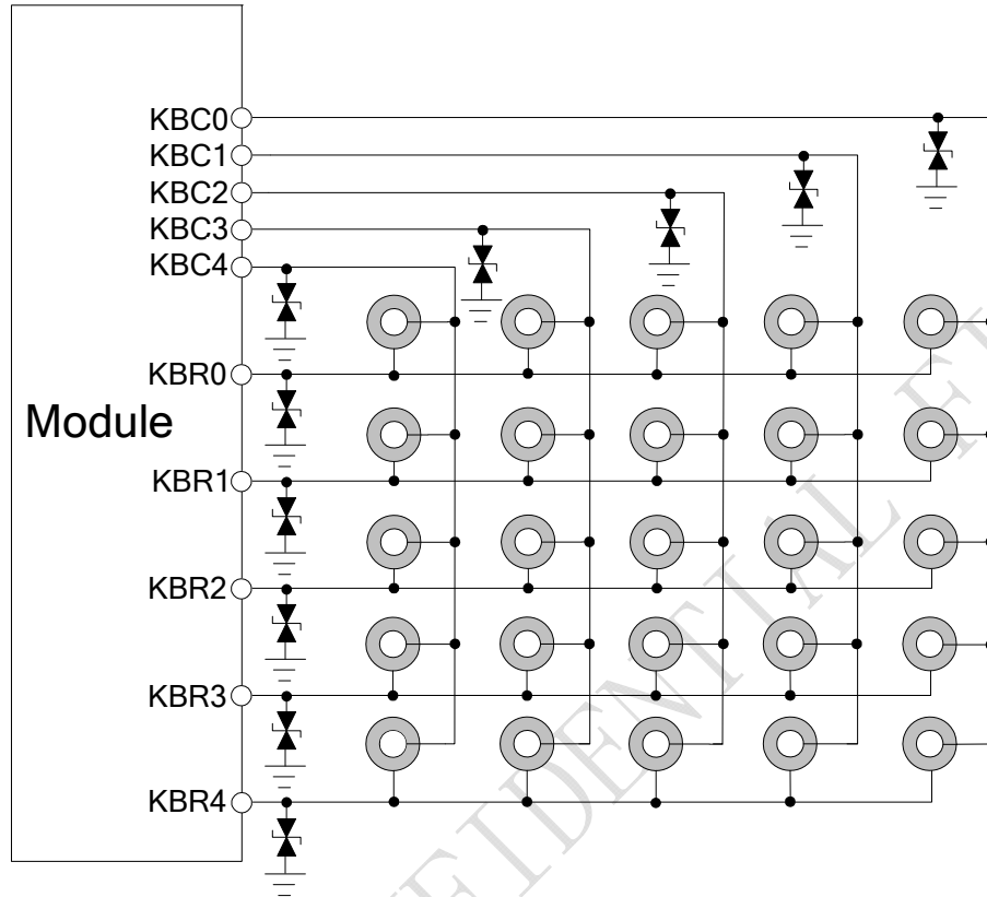
Figure 24: Reference circuit
