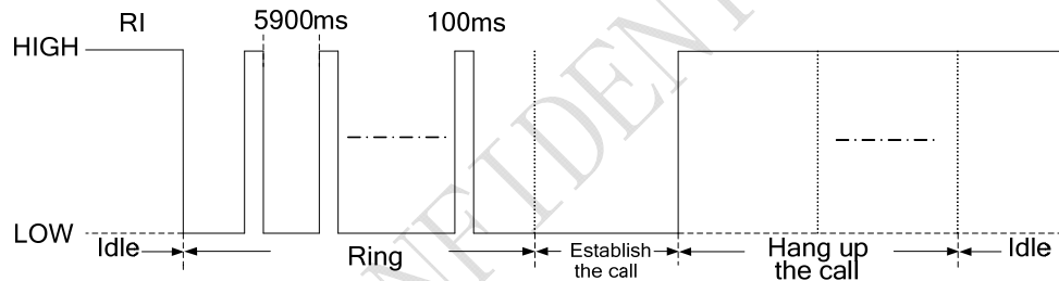
Figure 19: RI behaviour in FULL Modem
