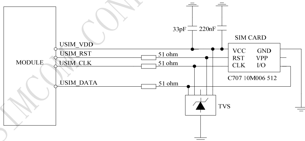
Figure 22: USIM interface reference circuit
