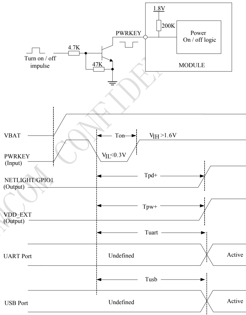
Figure 14: Power on Timing Sequence
