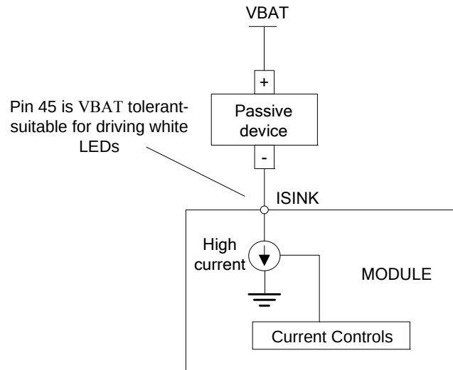
Figure 37: Current drive
