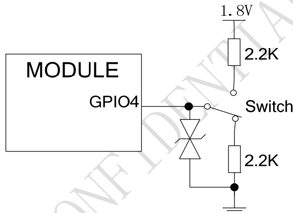
Figure 27: Flight mode switch
