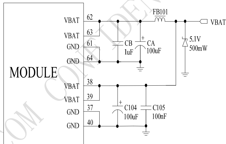
Figure 8: VBAT input application circuit
