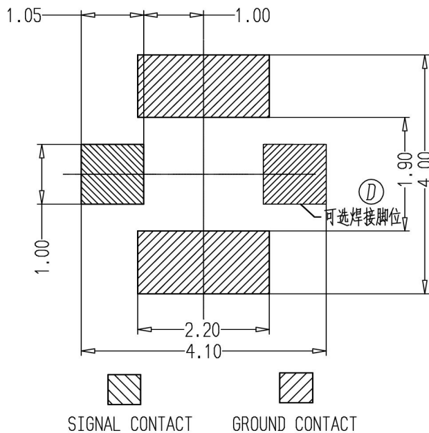
P.C.B DIMENSION (TOP VIEW) (TOLERRANCE ±0.05)
