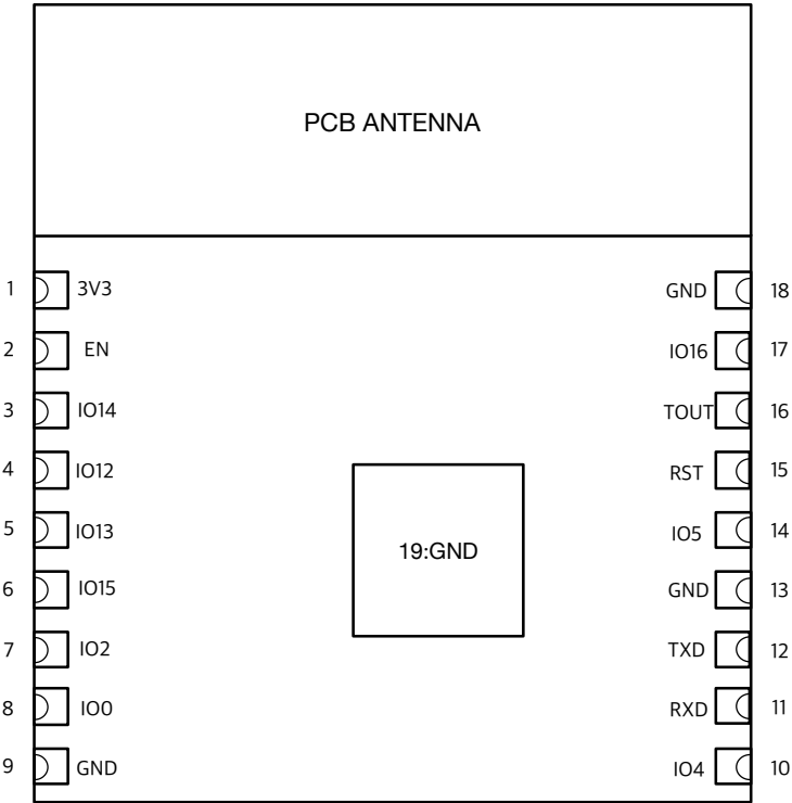
Figure 2-1. ESP-WROOM-02D Pin Layout (Top View)
